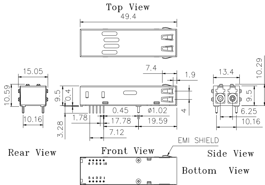
TRSL-73160EG / TRSL-73160CEG
